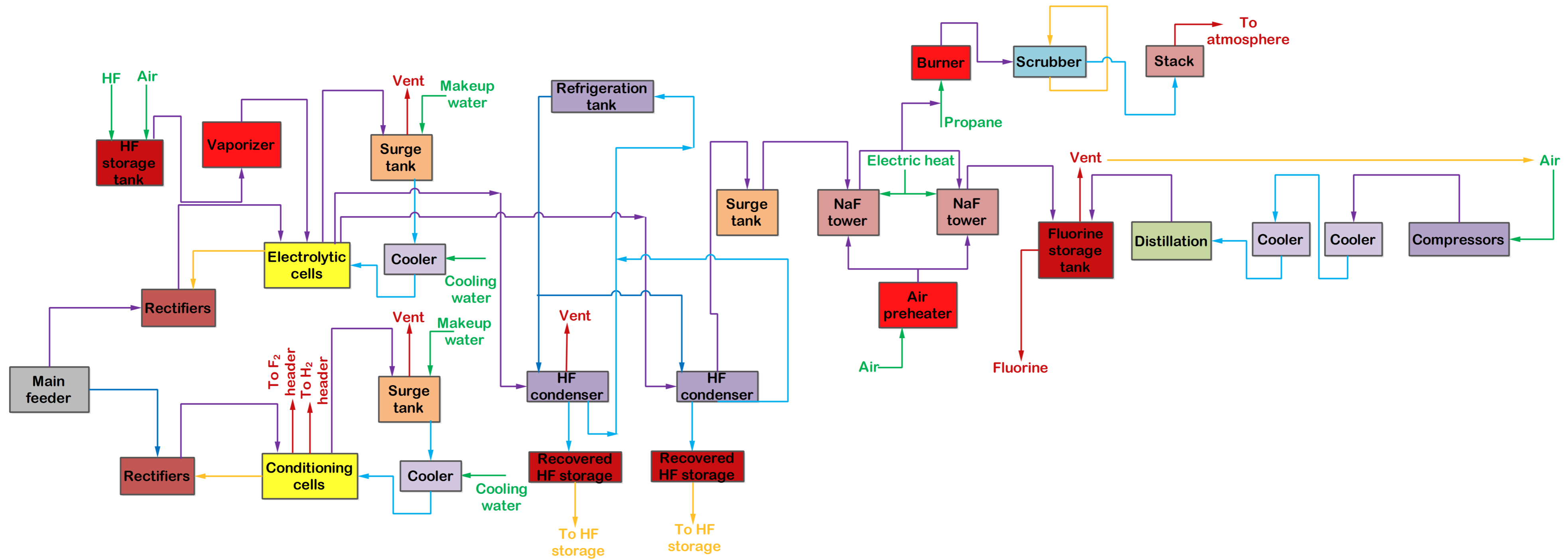
Figure: Manufacture of Fluorine by electrolysis of \text{KHF}_2
